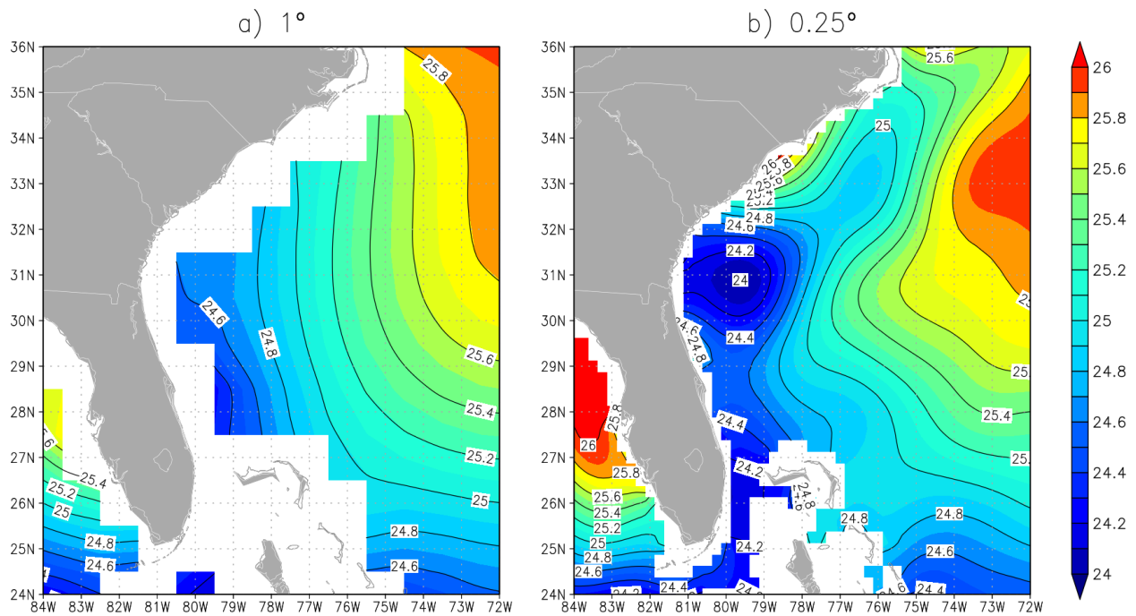
Figure 1. The winter (January-March) density of the Gulf Stream at 10 m depth for the 2005-2017 decade as represented by a) one-degree resolution and b) quarter-degree resolution.
