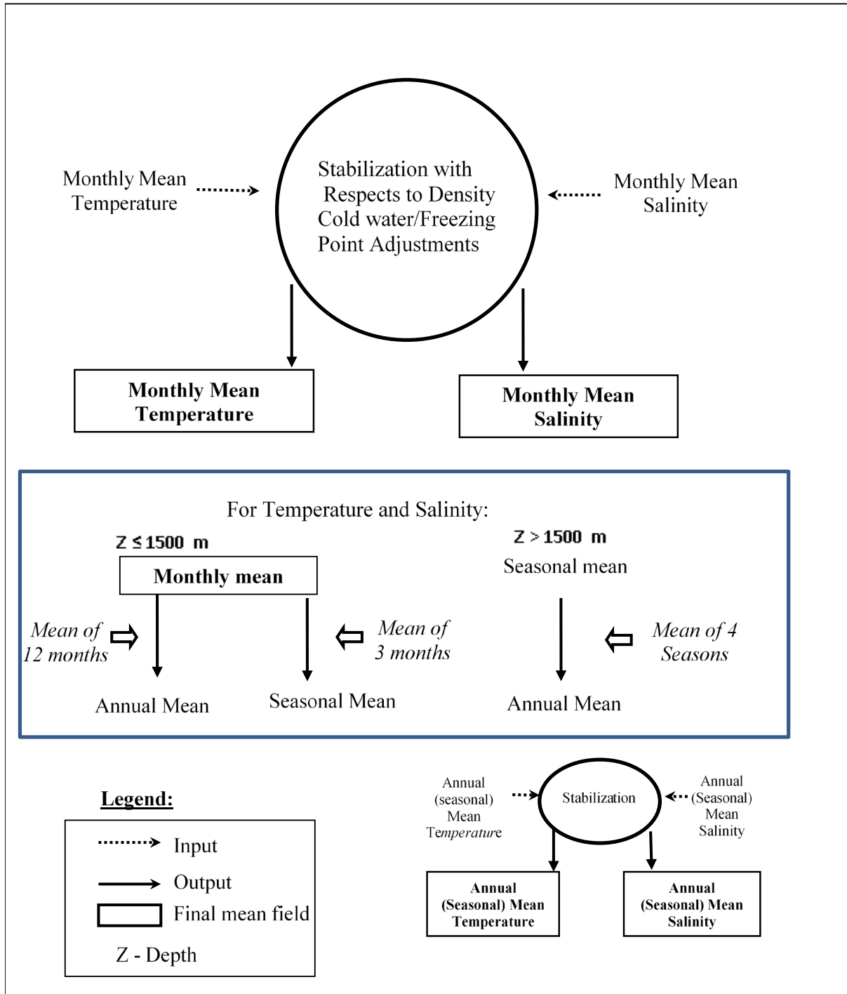
Figure 3. Scheme used in computing “all-data” annual, seasonal, and monthly objectively analyzed means for temperature, salinity, and density.
