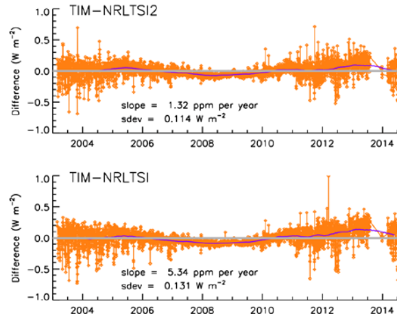
Figure 15: Differences in daily total solar irradiance that the algorithm calculates (according to NRLTSI2) with TIM observations (upper) and the original NRLTSI model (lower).
