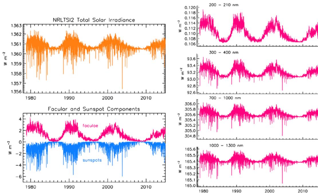
Figure 6: Total solar irradiance reconstructed with the NRLTSI2 model algorithm (upper), and the corresponding individual facular and sunspot contributions to the total solar irradiance variations (lower).
