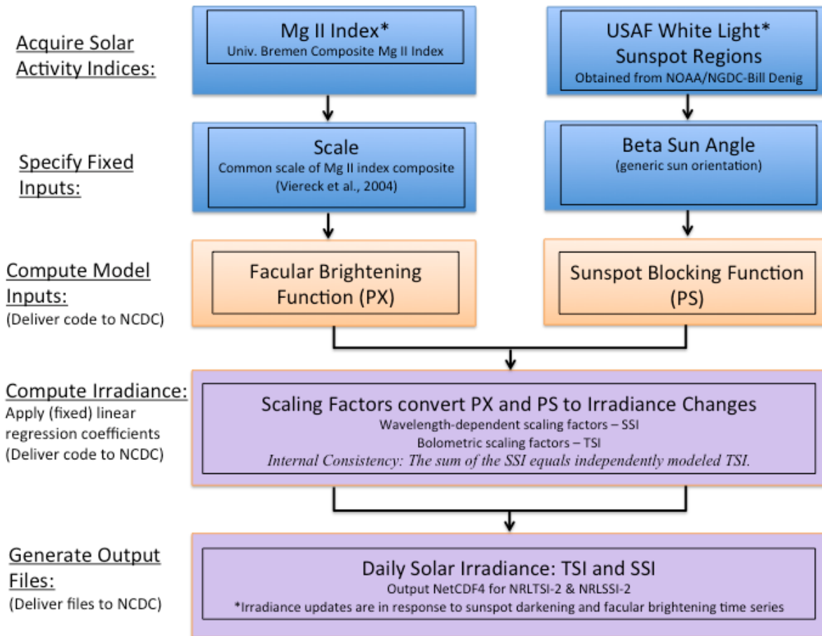
Figure 1: Flow diagram of the algorithm processing.
