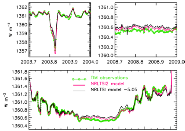
Figure 14: The total solar irradiance time series calculated by the algorithm (NRLTSI2 model) is compared with TIM observations during solar rotation (upper panel) and during the solar cycle (middle and lower panels). The middle panel is monthly-average data.
