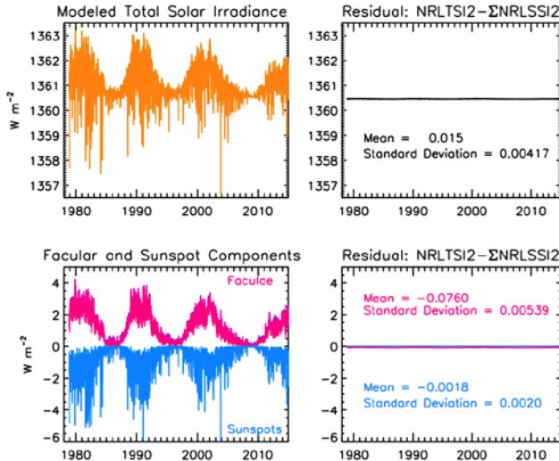
Figure 8: Comparison of NRLTSI2 total solar irradiance variations calculated by the algorithm, with the integral of the NRLSSI2 spectra also calculated by the algorithm (upper), and similar comparisons of their respective facular and sunspot components (lower).
