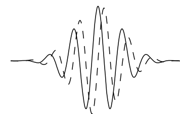
Morlet 6.00
