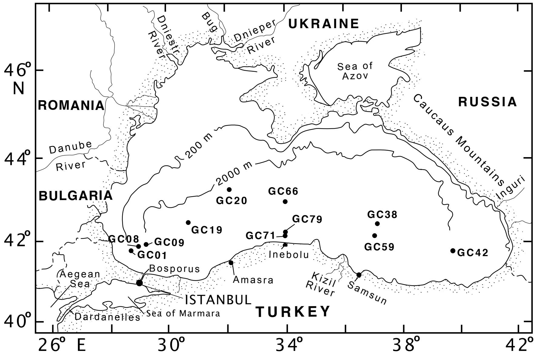
Locations of Black Sea core sites
