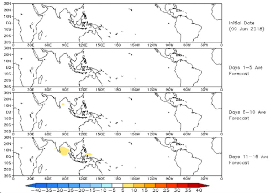
OLR prediction of MJO-related anomalies using CA model reconstruction by RMM1 & RMM2 (09 Jun 2018)
