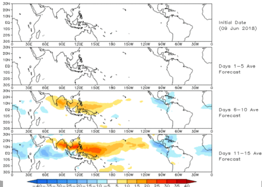
Prediction of MJO-related anomalies using GEFS operational forecast Initial date: 09 Jun 2018 OLR
