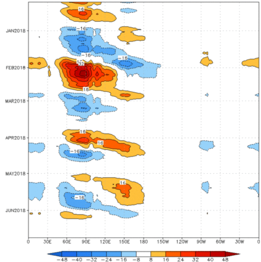
Reconstructed anomaly field associated with the MJO using RMM1 & RMM2 OLR [7.5°S,7.5°N] (cint:4Wm -2 ) Period:08-Dec-2017 to 09-Jun-2018 The unfilled contours are CA forecast reconstructed anomaly for 15 days
