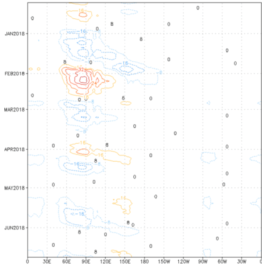
Reconstructed anomaly field associated with the MJO using RMM1 & RMM2 OLR [7.5°S,7.5°N] (cont:4Wm -2 ) Period:08-Dec-2017 to 09-Jun-2018 The unfilled contours are GEFS forecast reconstructed anomaly for 15 days
