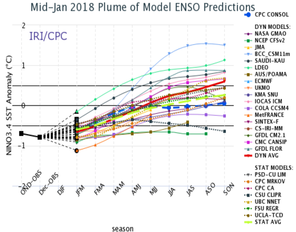
Figure provided by the International Research Institute (IRI) for Climate and Society (updated 18 January 2018).
