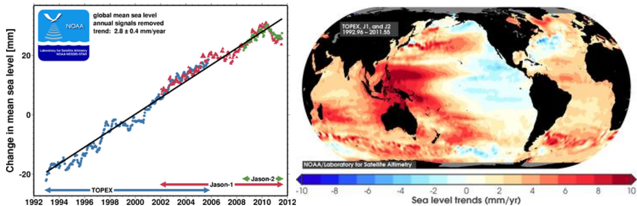
Figures 8&9: (Left) Change in global mean sea-level (mm) from 1992-2011; (Right) regional sea-level trends ( \pm mm/yr) from 1992-2011.
