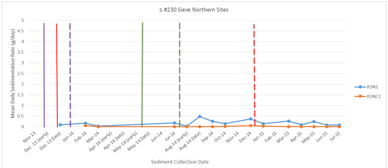
Figure 105. Daily sedimentation rates at northern outer reef sites for coarse-grain sediment (≥ #230 sieve) from baseline through post-construction surveys. The solid purple line on November 20, 2013 represents the first day of dredging by the hopper dredge Terrapin Island. The solid red line represents the first day of dredging for the Texas. The dotted purple line signifies the departure of the Terrapin Island (12/27/2013). The solid green line represents the first day of dredging for the Liberty Island (05/14/2014), and the green dotted line is the last day of dredging for the Liberty Island (07/03/2014). The red dash line represents the last day offshore dredging for Dredge Texas (12/23/2014). Sediment samples were not collected, until after the commencement of dredge operations, from R3N1 and R3NC1 due to environmental conditions that created unsafe diving conditions as well as hazardous conditions that prevented safe passage to the sites.
