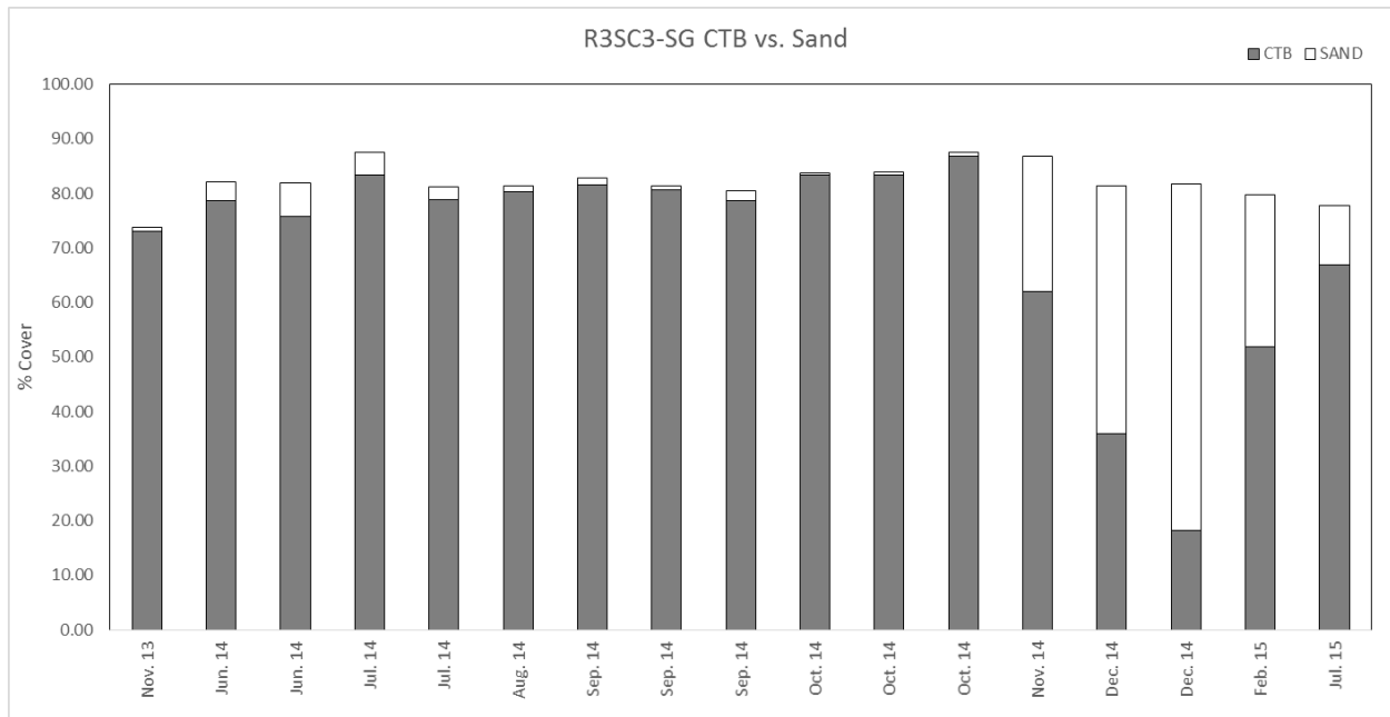
Figure 96. R3SC3-SG CTB (crustose, turf, and bare) and sand data analysis based on video transect analysis. First column of the figure represents baseline analysis, and last column on the figure represents post-construction analysis.
