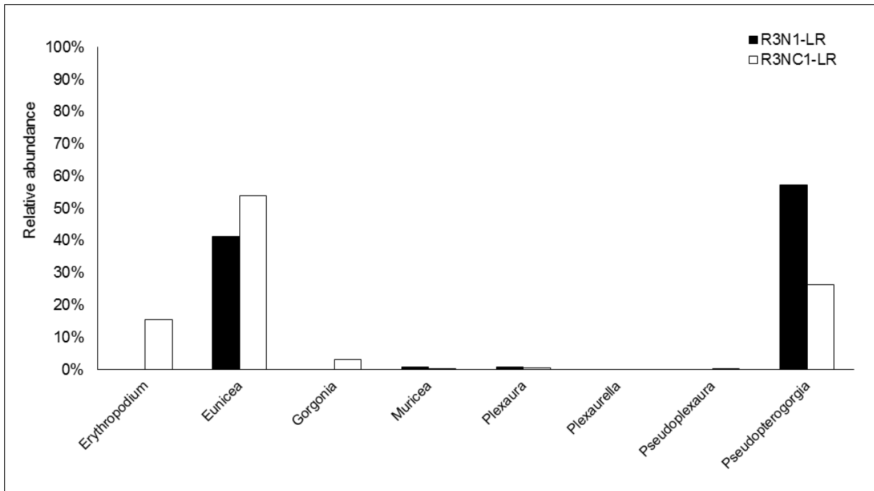
Figure 56. Relative abundance of octocorals at northern outer reef sites during baseline surveys.
