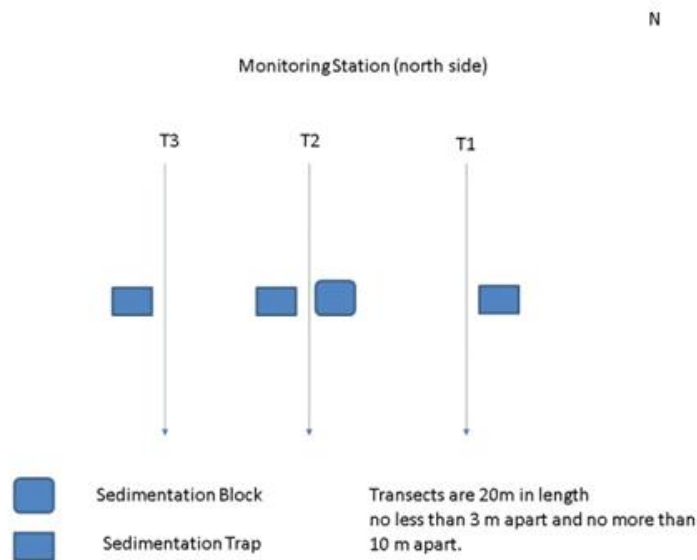
Figure 2. Middle and outer reef monitoring site layout.
