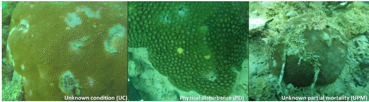
Figure 8. Photographs of stress indicators collected during compliance and post-construction surveys.
