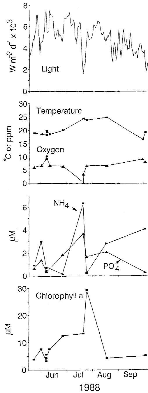
Time course of light, temperature, oxygen, ammonium, phosphate, and chlorophyll in water of Waquoit Bay, summer 1988. Modified from Costa et al. (in press).
