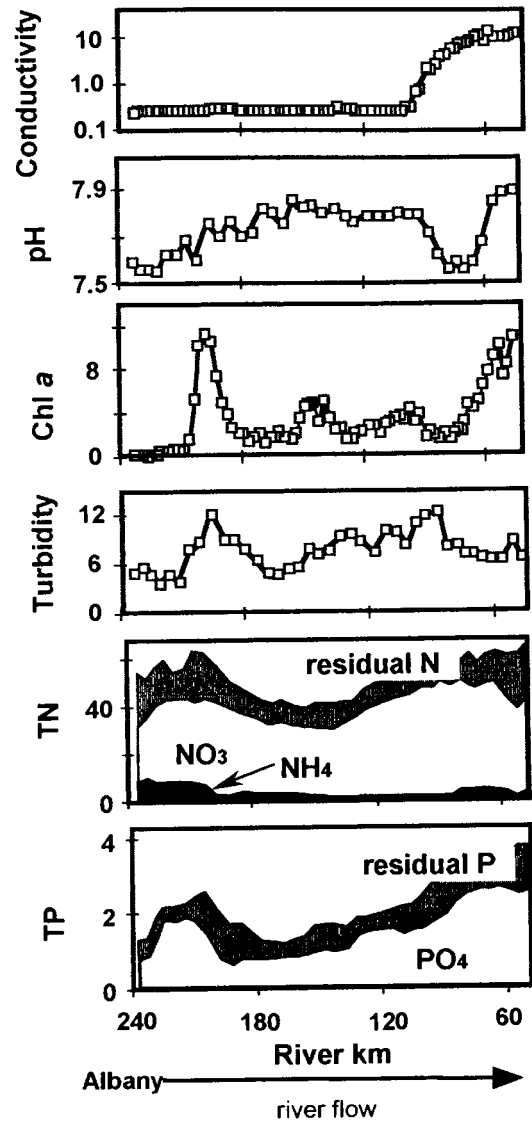
Spatial variation in selected variables for a representative transect taken in early September 1996. Transects run km 240 (Albany) downstream to km 40. For each variable samples were taken every 2 to 4 km. Units are, conductivity—(note log scale); pH—normal pH units; chlorophyll a — l^{-1} ; turbidity— NTU; N and P— \mu M. For both N and P the per line represents total N and total P. “Other N” is TN minus DIN ( NH_4 plus NO_3 ); For P, “Other P” is TP minus phosphate.
