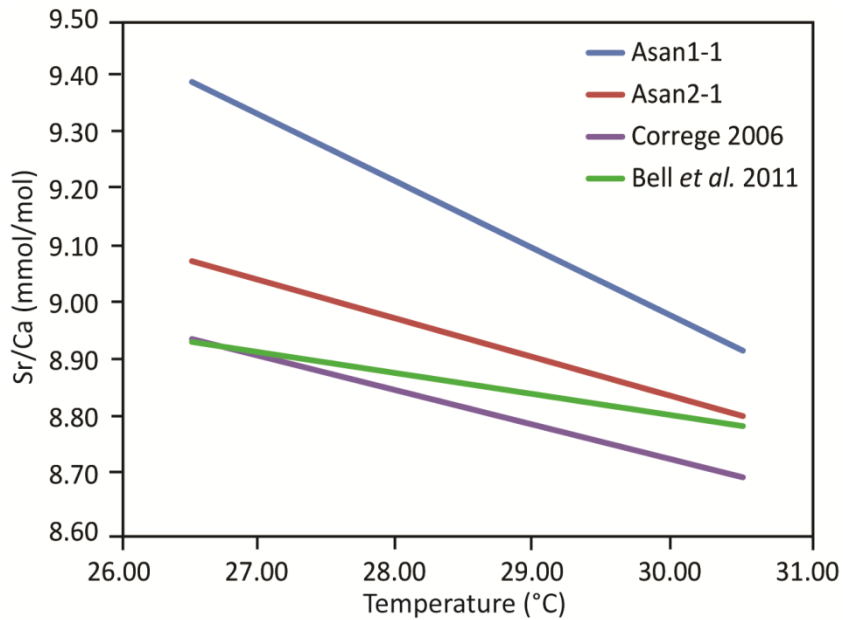
Figure 3.11 Sr/Ca-SST calibration equations for Asan1-1 and Asan2-1 monthly datasets compared with the average Porites equation presented by Correge (2006) and that from Bell et al. (2011a).
