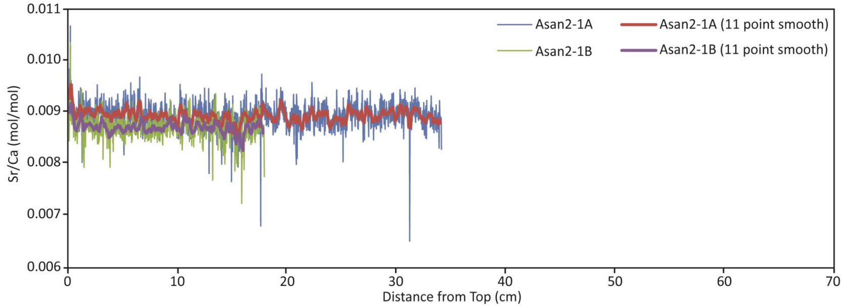
Figure C-4 High-resolution Sr/Ca values from Asan2-1 as measured at distances from the top of the core (most recent skeletal material) to the bottom (oldest skeletal material). A and B indicate two separate transects along which Sr/Ca was measured as replicates. The thicker lines indicate the 11-point moving average of the original 0.22mm-resolution data set.
