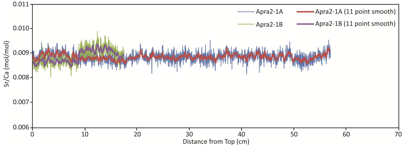
Figure C-2 High-resolution Sr/Ca values from Apra2-1 as measured at distances from the top of the core (most recent skeletal material) to the bottom (oldest skeletal material). A and B indicate two separate transects along which Sr/Ca was measured as replicates. The thicker lines indicate the 11-point moving average of the original 0.22mm-resolution data set.
