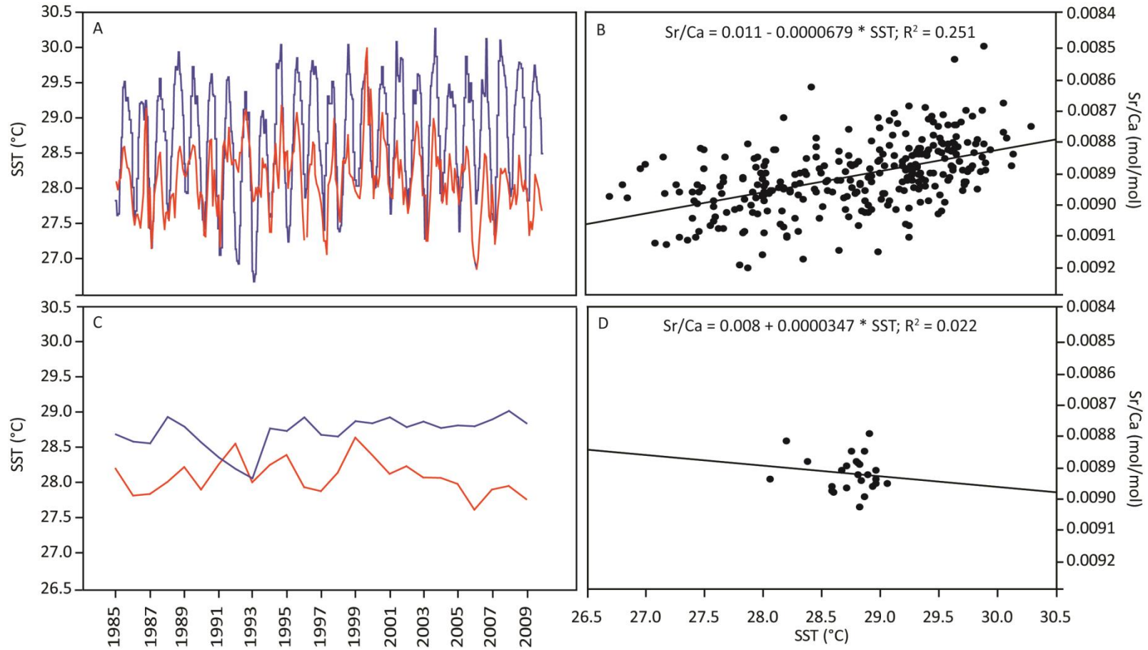
Figure 3.9 Asan2-1 Sr/Ca-SST analysis. A.) 1985-2010 monthly time series for SST (blue line) and Sr/Ca (red line) and B.) a regression plot of the same time series. C.) 1985-2010 annual time series for SST (blue line) and Sr/Ca (red line) and D.) a regression plot of the same time series.
