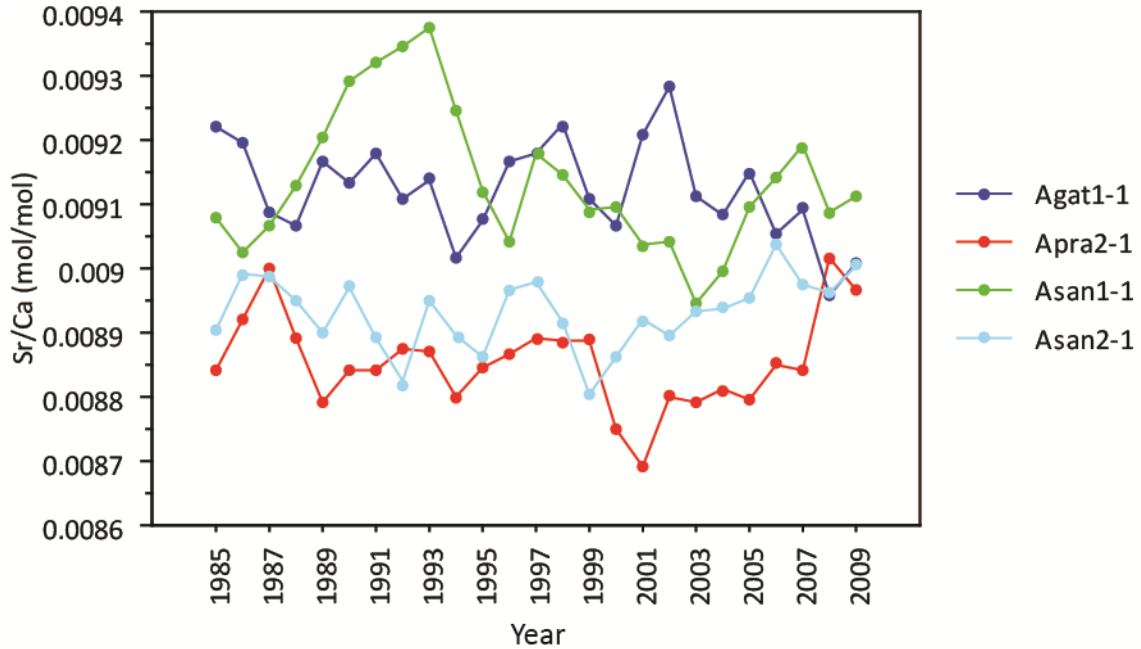
Figure 3.5 Annual Sr/Ca measurements 1985-2010
