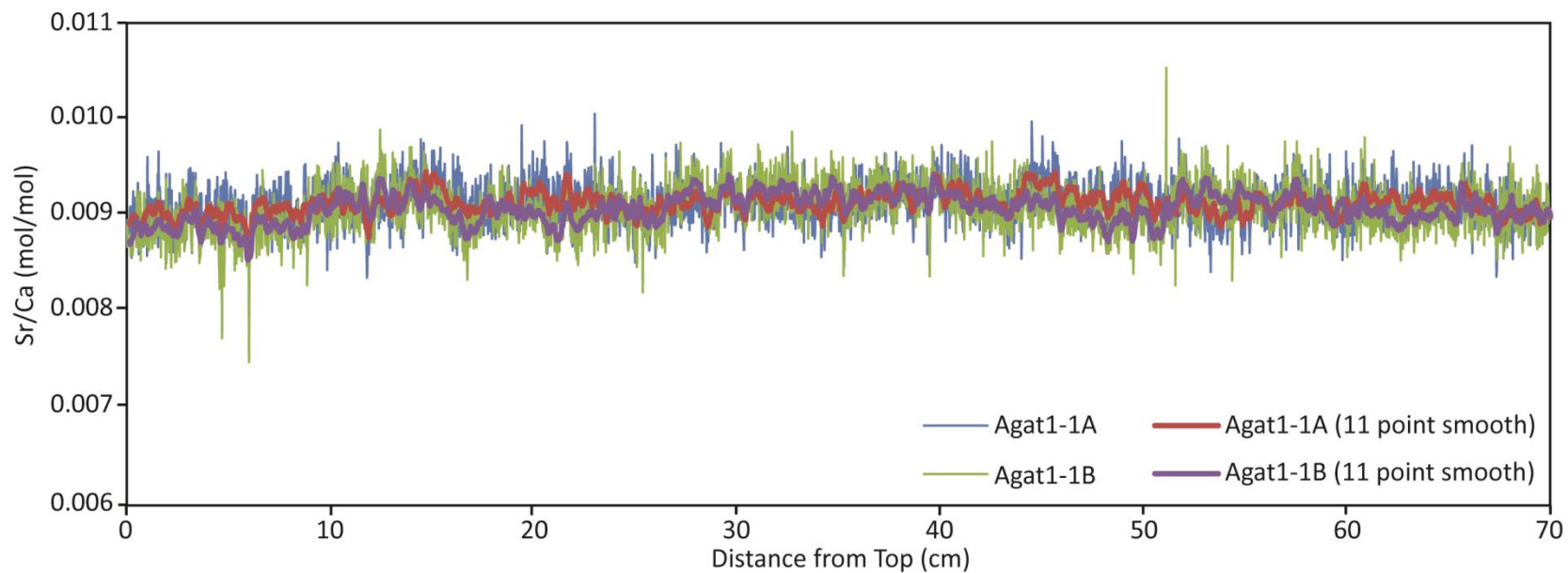
Figure C-1 High-resolution Sr/Ca values from Agat1-1 for the first 70 cm of each transect as measured at distances from the top of the core (most recent skeletal material) to the bottom (oldest skeletal material). A and B indicate two separate transects along which Sr/Ca was measured as replicates. The thicker lines indicate the 11-point moving average of the original 0.22mm-resolution data set.
