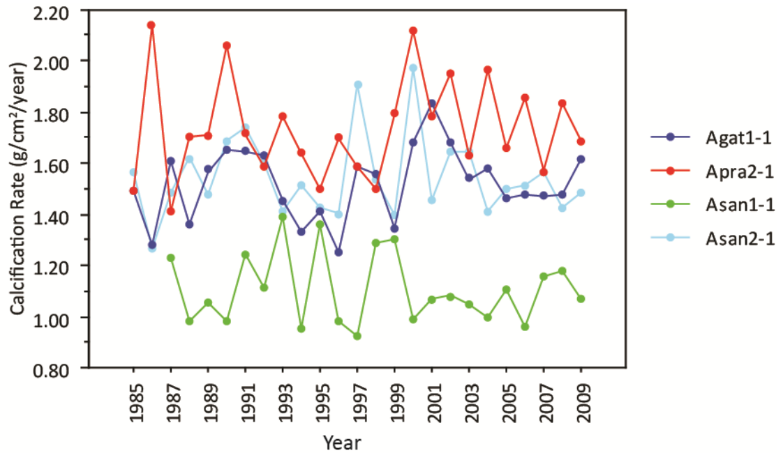
Figure 3.4 Annual calcification rates 1985-2010
