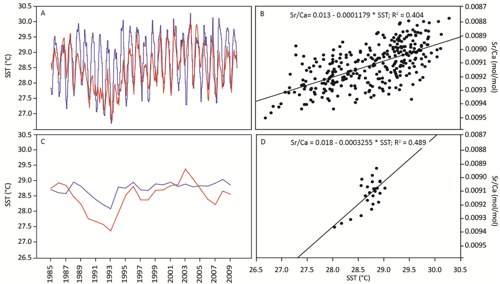
Figure 3.8 Asan1-1 Sr/Ca-SST analysis. A.) 1985-2010 monthly time series for SST (blue line) and Sr/Ca (red line) and B.) a regression plot of the same time series. C.) 1985-2010 annual time series for SST (blue line) and Sr/Ca (red line) and D.) a regression plot of the same time series.
