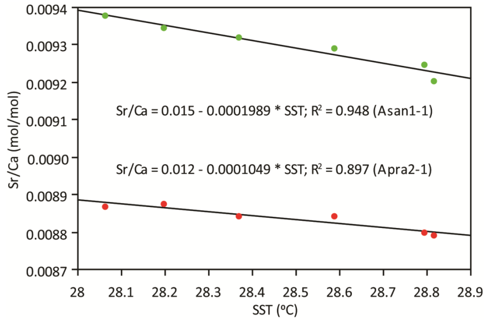
Figure 3.10 Regression plots for annual Sr/Ca and SST 1989-1994 for Apra2-1 and Asan1-1.
