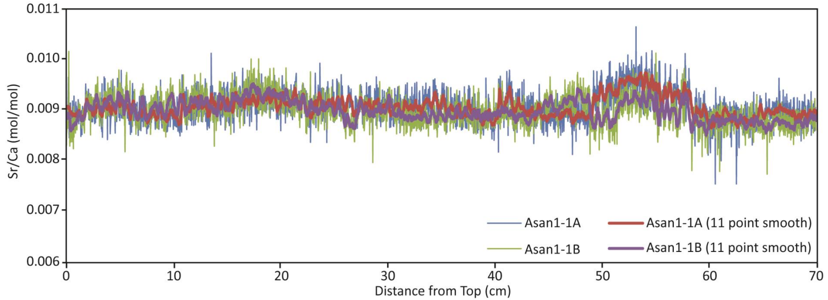
Figure C-3 High-resolution Sr/Ca values from Asan1-1 for the first 70 cm of each transect as measured at distances from the top of the core (most recent skeletal material) to the bottom (oldest skeletal material). A and B indicate two separate transects along which Sr/Ca was measured as replicates. The thicker lines indicate the 11-point moving average of the original 0.22mm-resolution data set.
