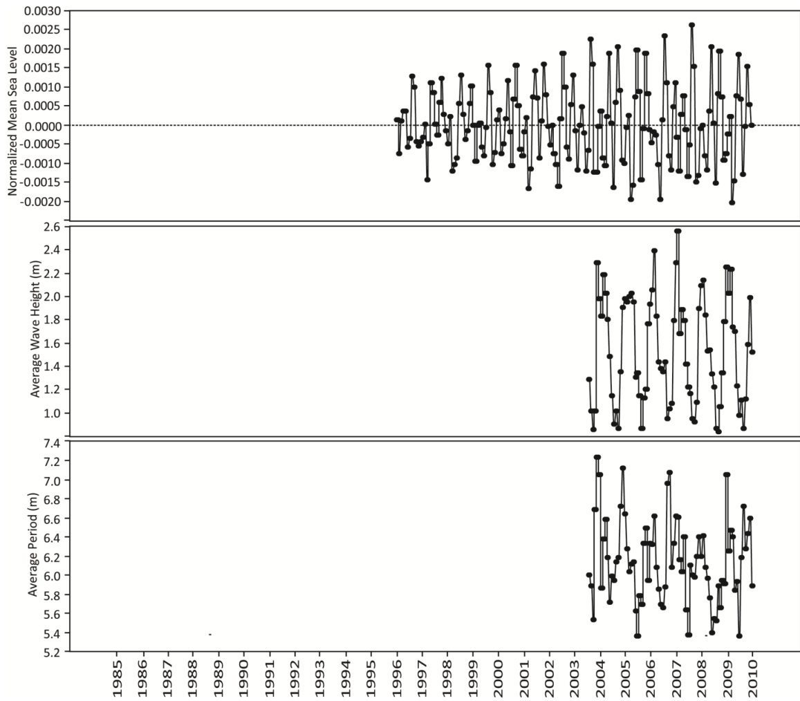
Figure 3.13 Environmental time series for mean sea level, wave height and average wave period 1985-2010
