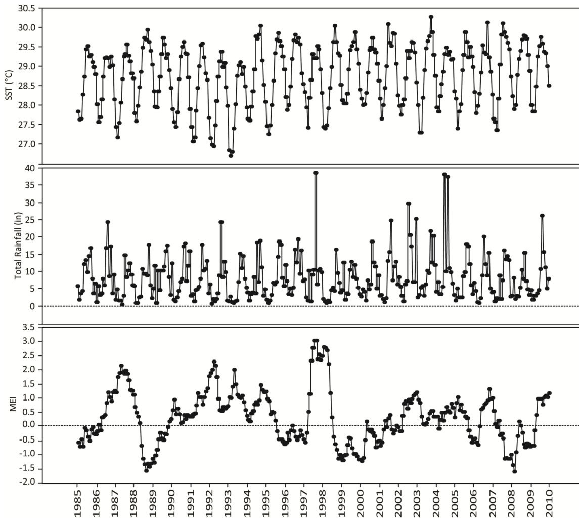
Figure 3.12 Environmental time series for SST, total rainfall, and MEI 1985-2010
