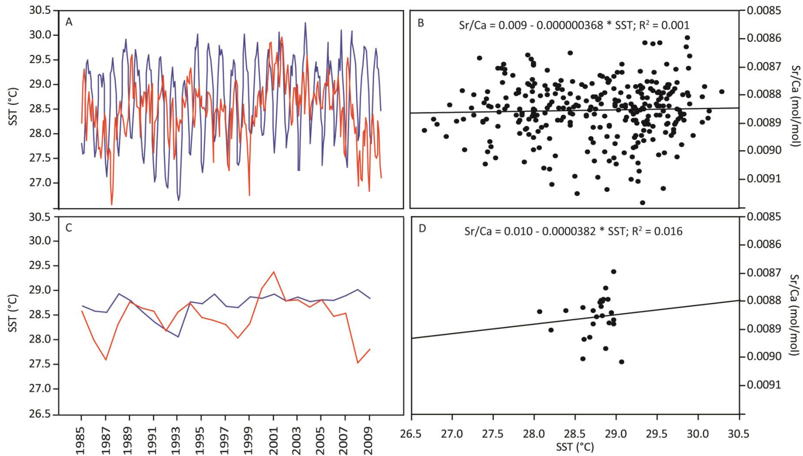
Figure 3.7 Apra2-1 Sr/Ca-SST analysis. A.) 1985-2010 monthly time series for SST (blue line) and Sr/Ca (red line) and B.) a regression plot of the same time series. C.) 1985-2010 annual time series for SST (blue line) and Sr/Ca (red line) and D.) a regression plot of the same time series.
