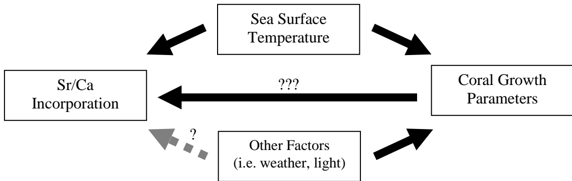
Figure 1.1 Relationship model between SST, Sr/Ca, and coral growth. Arrows indicate dependencies between factors (solid = direct effect, dashed = indirect effect). Question marks indicate potential relationships which will be assessed in the proposed study.
