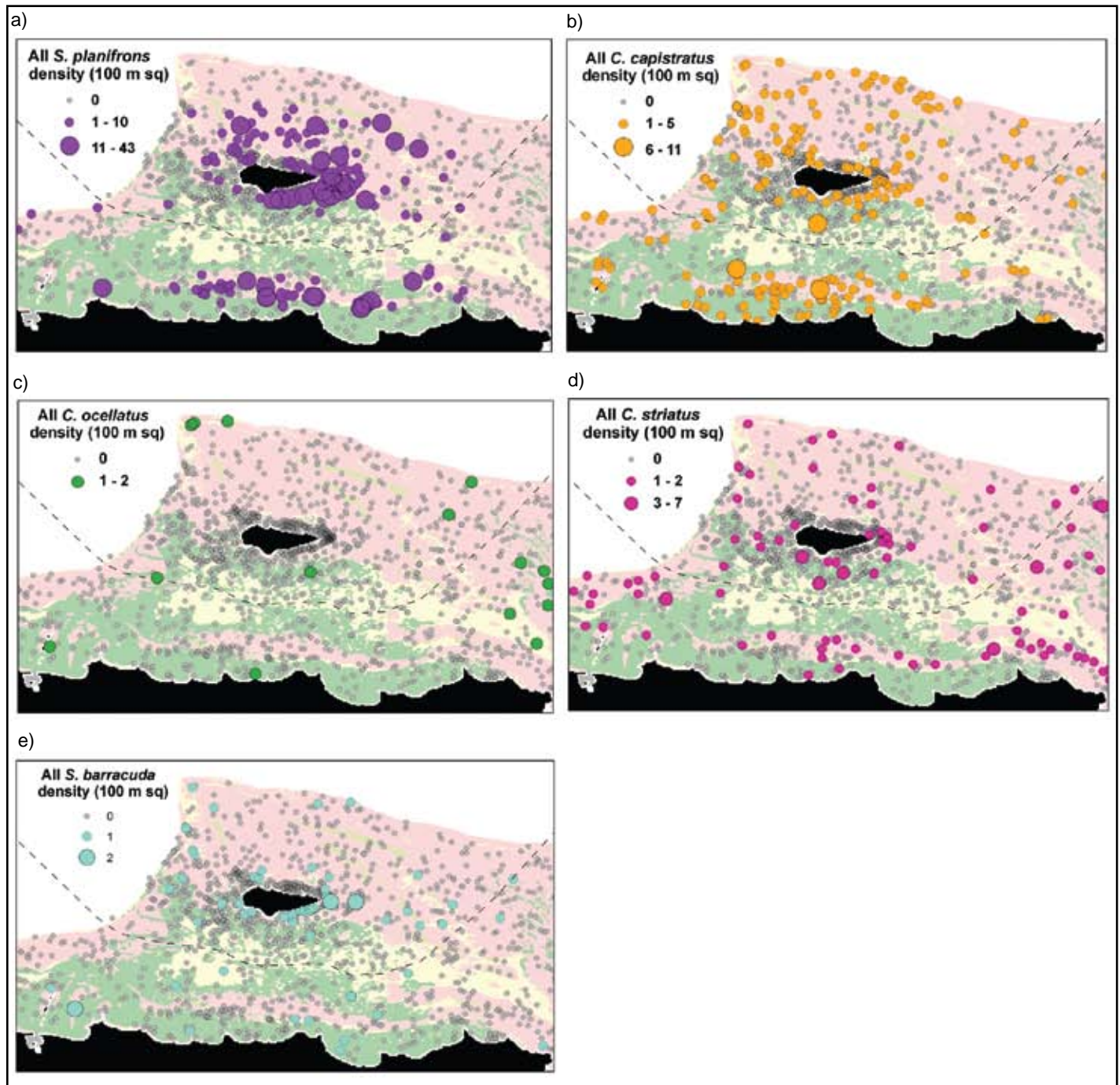
Figure D3. Spatial distributions of juvenile and adult: (a) threespot damselfish ( Stegastes planifrons ), (b) four-eye butterflyfish ( Chaetodon capistratus ), (c) spotfin butterflyfish ( Chaetodon ocellatus ), (d) banded butterflyfish ( Chaetodon striatus ) and (e) great barracuda ( Sphyraena barracuda ) in northeastern St. Croix.
