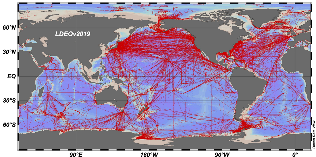
Fig. 1. Location of LDEO V2019 master database of sea surface pCO 2 observations.
