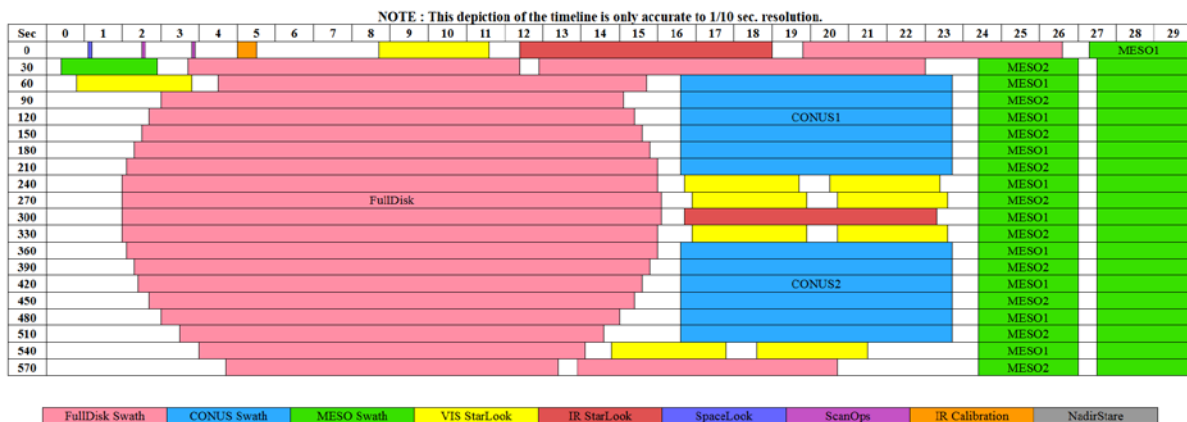
Figure 4: ABI 10-Minute Flex Mode (scan mode 6) timeline diagram. Timeline diagrams (often called “time-time diagrams”) like this one depict the observations of ABI over 30 sections for each line, starting at the top. The numbers along the left are the starting times of each line, in seconds, from the beginning of the timeline. This timeline, for example, covers 10 min. Pink, blue, and green represent the time scanning the FD, CONUS, and mesoscale sectors, respectively. Autonomous space looks are also included as part of each pink FD swath. White represents the time when ABI slews the line-of-sight (LOS) between observations. Gray represents the time when ABI points at nadir, collecting no data.
