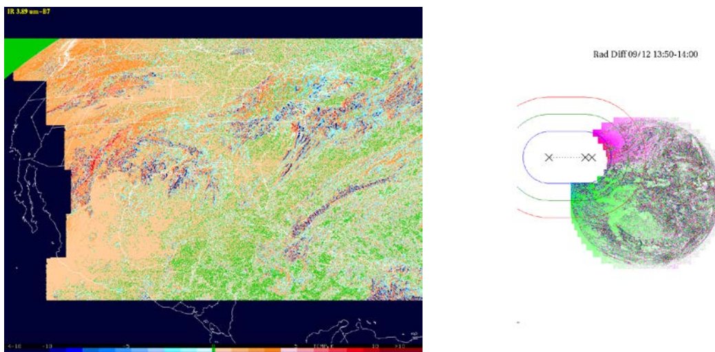
Figure 16: Example of IR stray light at night. The left panel shows the T_B ( 3.9\ \mu\text{m} ) change in five minutes, the closer to the Sun, the larger the T_B change. Note also that the colder the scene, the larger the T_B change, even for scene fairly far away from the Sun. The right panel illustrates the size of Restricted Zone (blue) and the Zone of Reduced Data Quality (ZRDQ, red).
